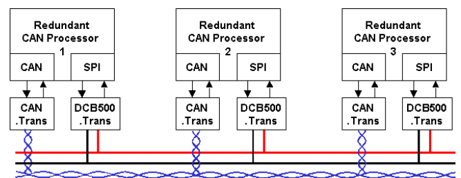
Figure 2 – Redundant CAN network
