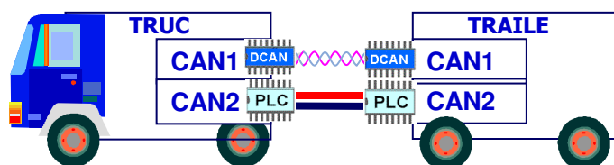
Figure 1.0 - Truck-Trailer Redundant communication
